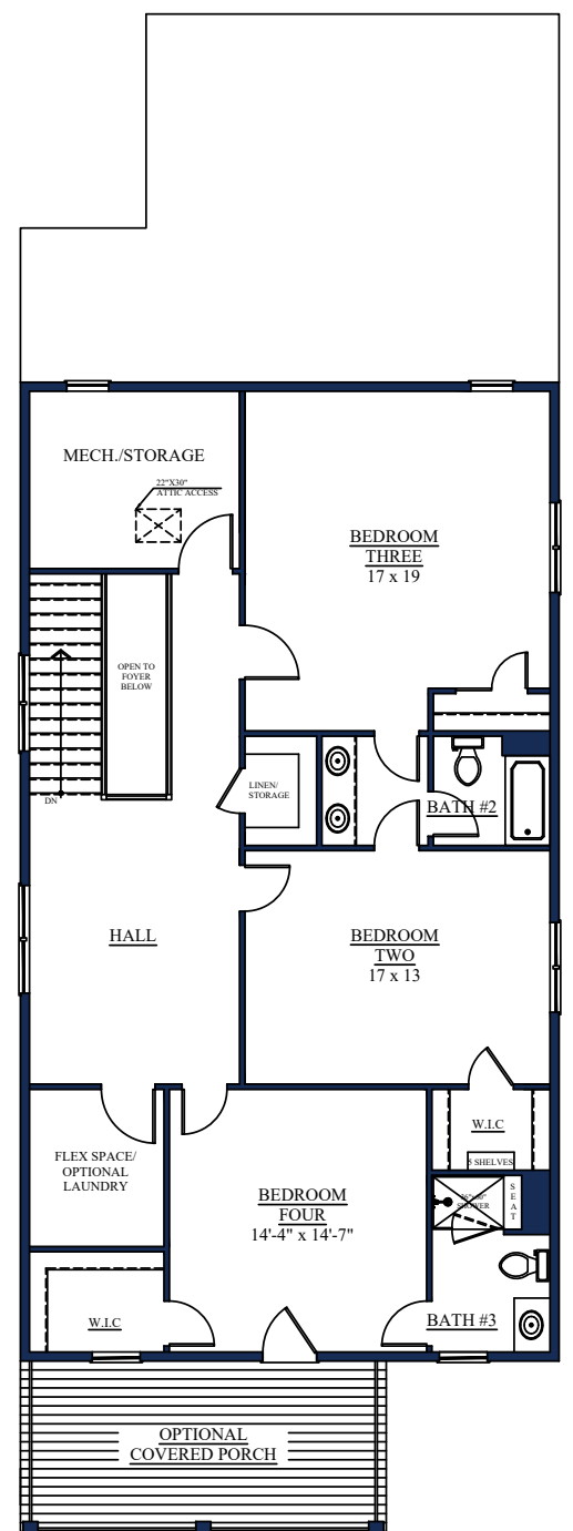
OPTIONAL UPPER LEVEL - THREE BEDROOM TWO BATH
