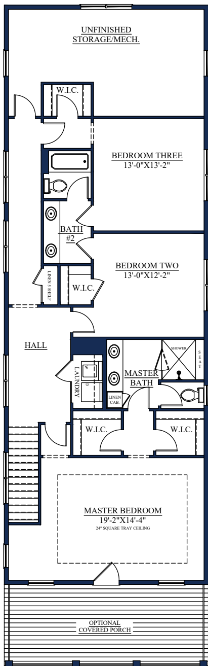
UPPER LEVEL - STANDARD THREE BEDROOM TWO BATH
