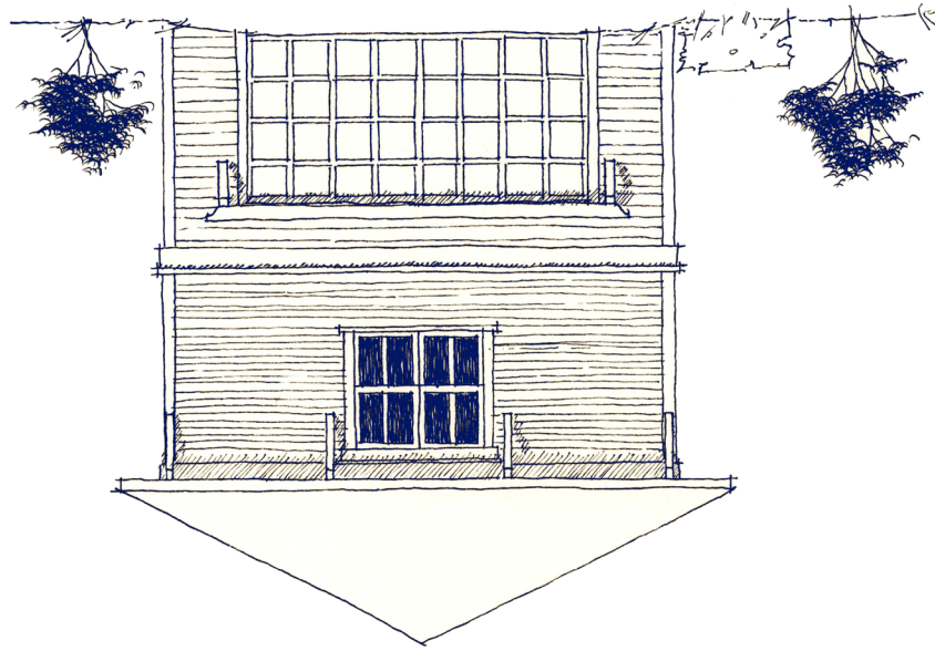
REAR ELEVATION A - STANDARD UPPER LEVEL
